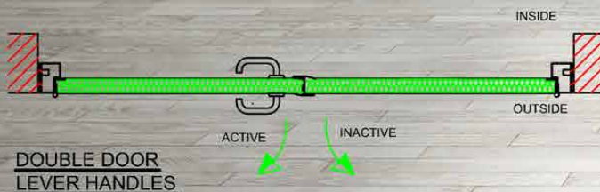
DOUBLE DOOR WITH LEVER HANDLE AND MORTICE SASH LOCK *EXTRA LOCKS CAN BE ADDED*
