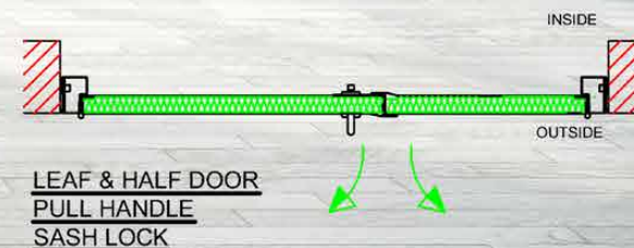
DOUBLE DOOR LEAF & HALF PULL HANDLE MORTICE SASH LOCK
