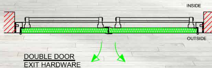
DOUBLE DOOR WITH FIRE EXIT HARDWARE
